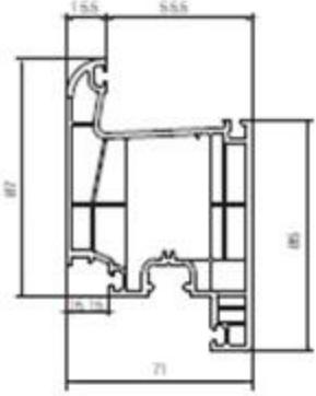
PRSC04 3 Contalı Kapı Profili Triple seal Opening Profile
