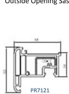
PR7121 30mm Çıta 30mm Glazing Bead
