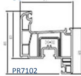
PR7102 Kanat Profili Sash Profile
