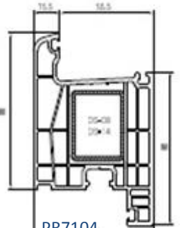
PR7104 Kilitli Kapı Profili Door Sash Profile
