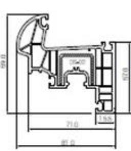
PRSC02 Kanat Profili Sash Profile
