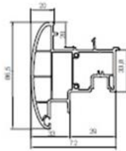
PRSC13 Stump Profili Stump Profile
