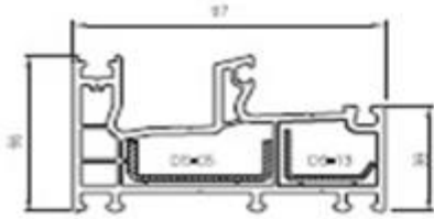
PRSY46 Fix Kasa Profili Fix Frame Profile
