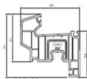
PR7107 Damaklı Kanat Profili Drainer Sash Profile
