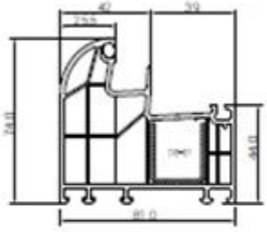
PRSC01 Kasa Profili Frame Profile
