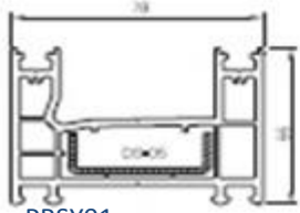
PRSY01 Kasa Profili Frame Profile
