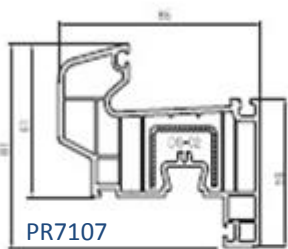
PR7107 Damaklı Kanat Profili Drainer Sash Profile
