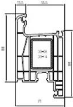
PR7104 Kilitli Kapı Profili Door Sash Profile
