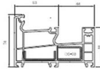
PRSY51 Dış Fix Kasa Profili Outside Fix Frame Profile
