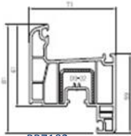
PR7102 Kanat Profili Sash Profile
