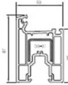
PRSY02 Kanat Profili Sash Profile
